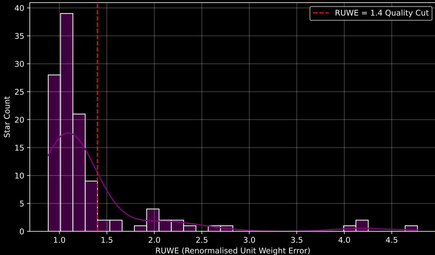
GALAH DR4 Field [2878] RUWE Distribution (n= 117)
