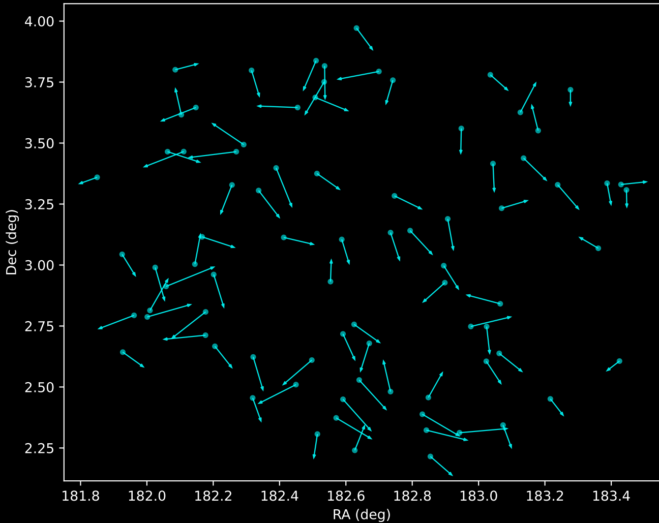
GALAH DR4 Noise Stream Proper Motion Vectors (n=82)
