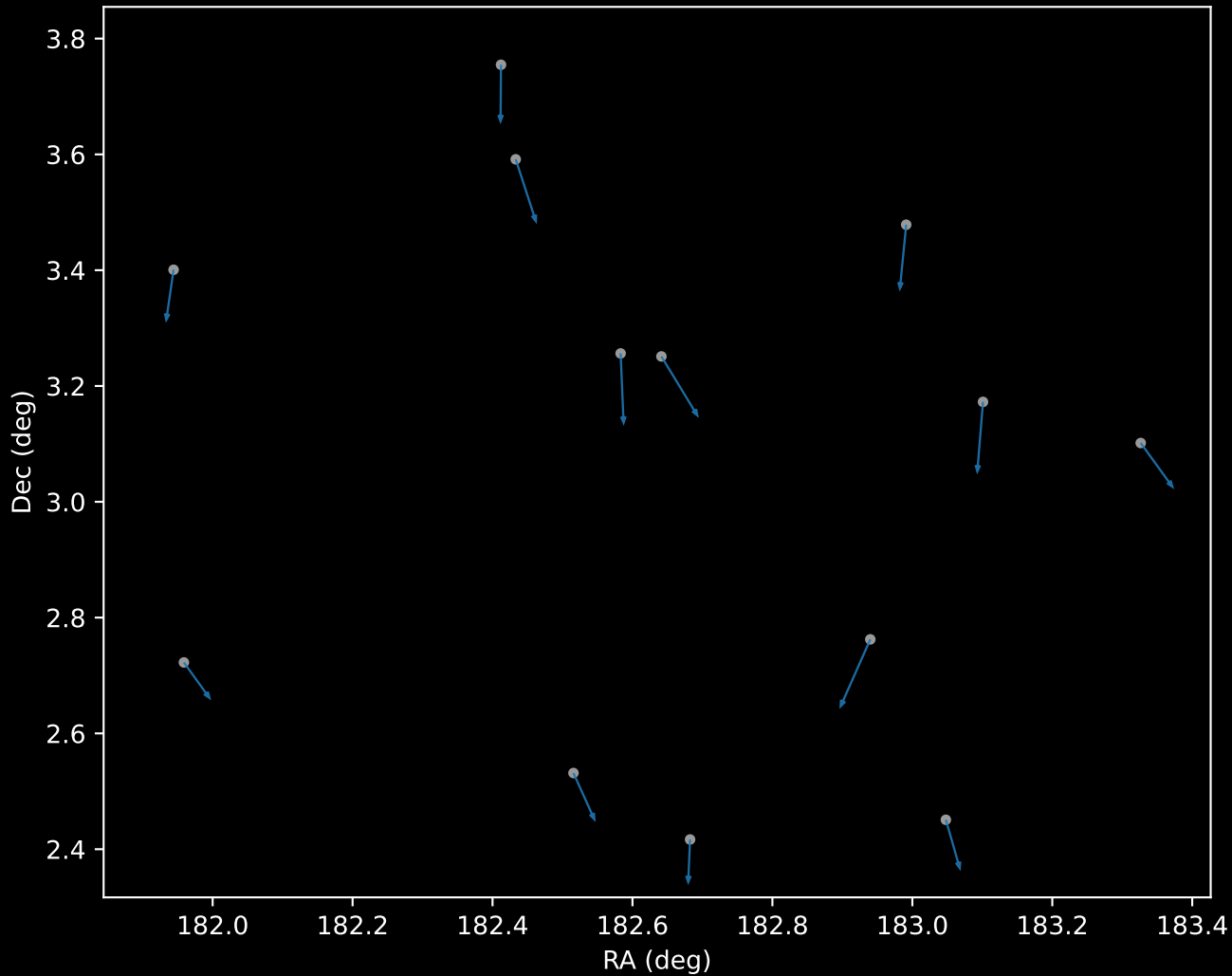
GALAH DR4 Cluster 0 Proper Motion Vectors (n=13)
