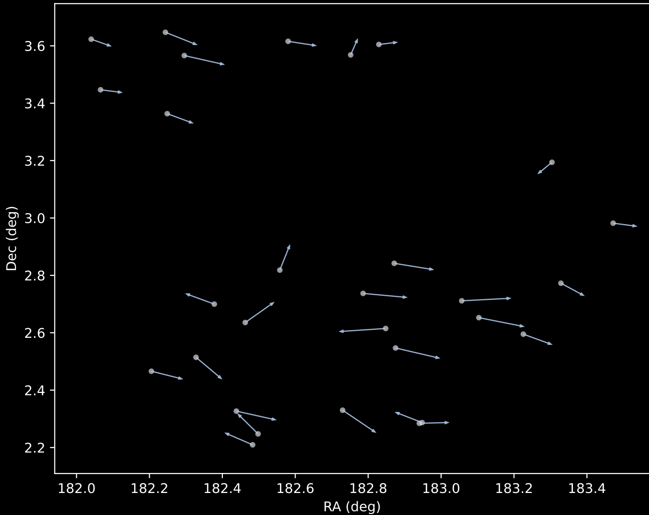
GALAH DR4 Cluster 1 Proper Motion Vectors (n=29)
