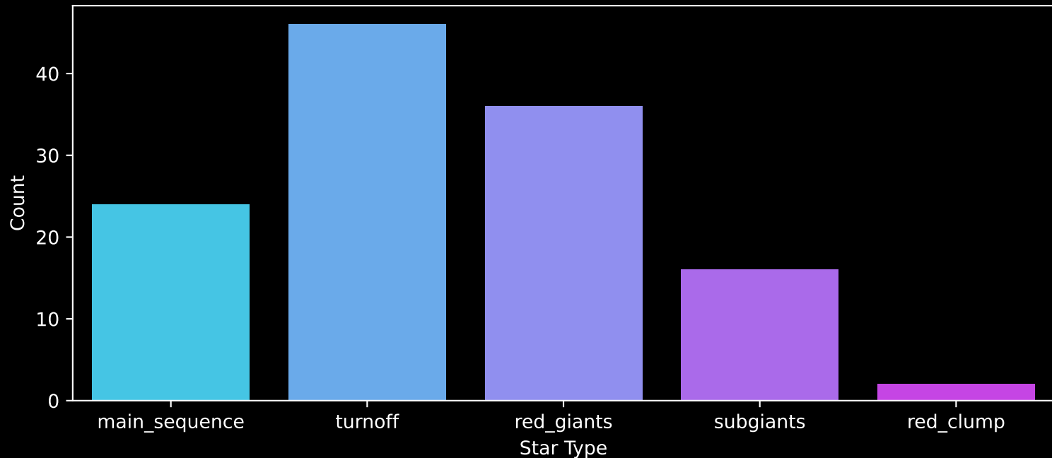
GALAH DR4 Field: [2878] Count plot of Star Type
